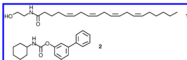
Figure 1. Chemical structures of anandamide ( 1 ) and URB524 ( 2 ).
