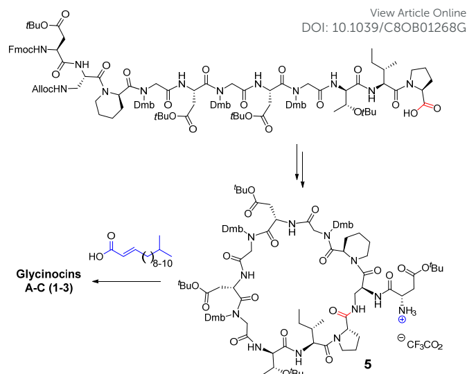
Figure 2. Previous total synthesis of glycinocins A-C (1-3).
