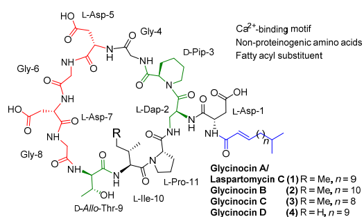
Figure 1. Glycinocins A-D with key structural features highlighted in red (Ca 2+ -binding motif), green (non-proteinogenic amino acids) and blue (fatty acyl moiety).
