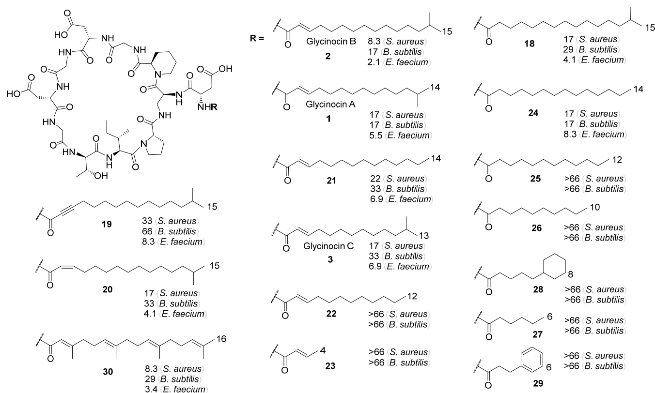
Figure 3. Antimicrobial activity of glycinocin analogues at 50 mg/L Ca^{2+} (MIC in \mu M ).
