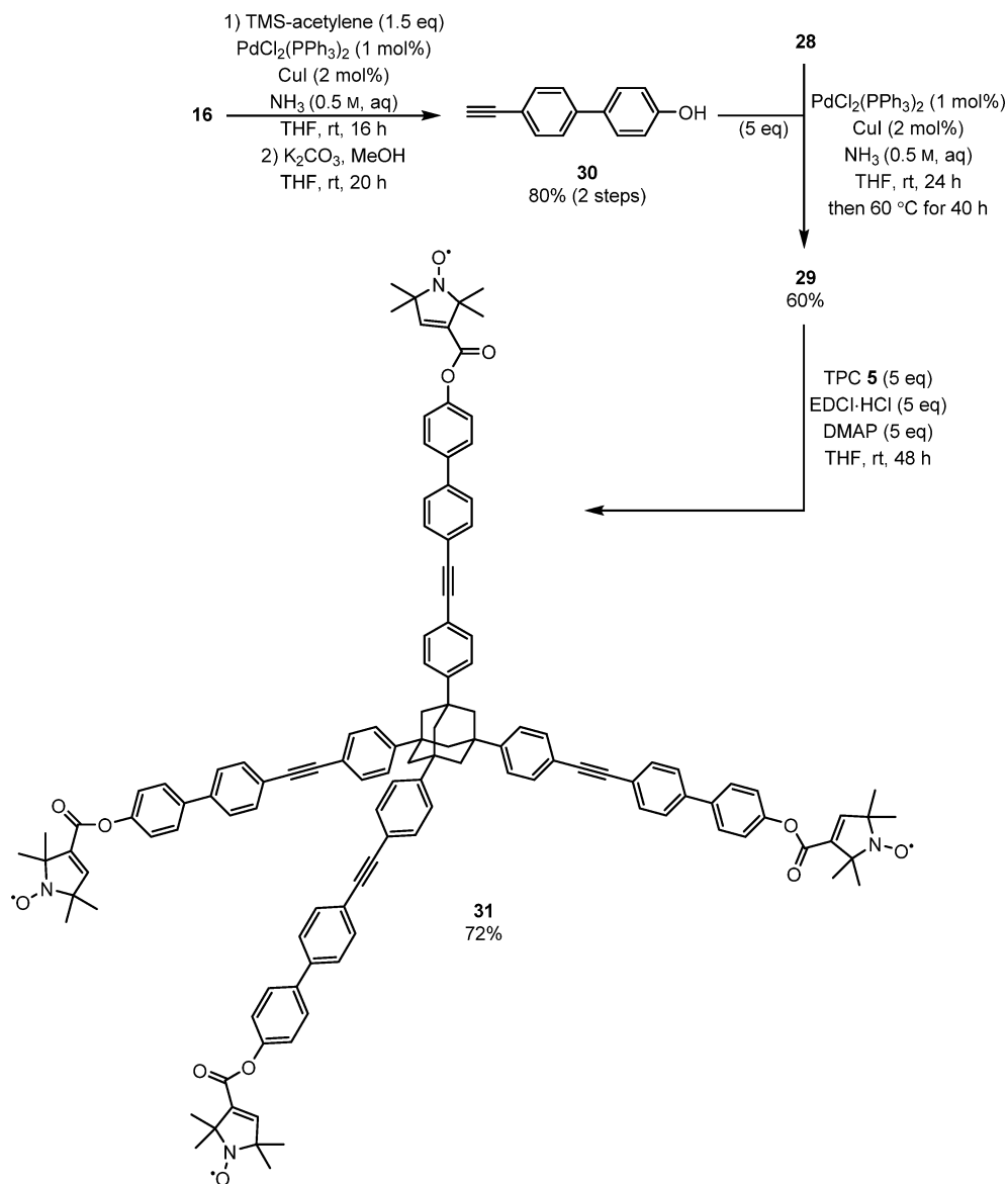
Scheme 11. Synthesis of Tetrahedral Tetradiradical 31
