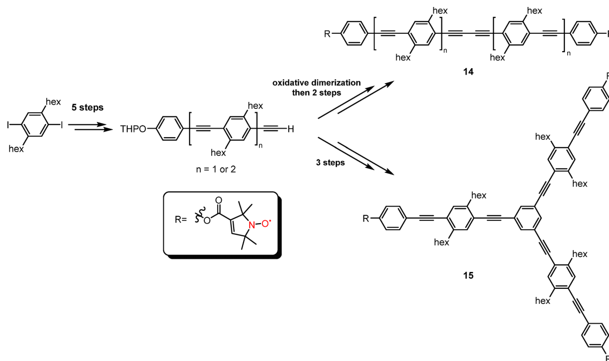
Scheme 3. Syntheses of Long Distance Polyradicals 4
