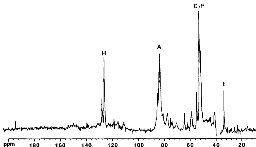
Fig. 2. ^{13}\text{C}\{^1\text{H}\} NMR difference spectrum of P. taeda extracellular lignin derived from [ 2\text{-}^{13}\text{C} ] phenylalanine; natural abundance resonances have been subtracted from the labelled spectrum. For explanation of substructures see Fig. 1.
