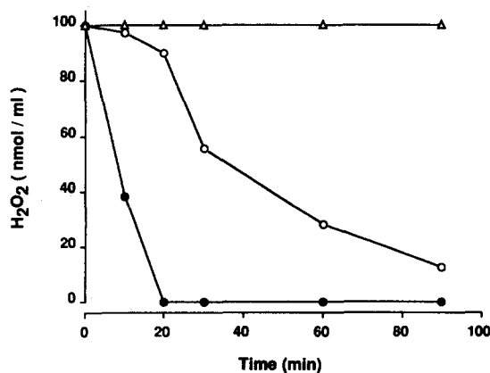
Fig. 4. Decomposition of hydrogen peroxide in solutions containing 20 mM KI/8% sucrose (○) and 20 mM KI/8% sucrose/horseradish peroxidase (●). Control experiments (△) were conducted using 8% sucrose solution alone.
