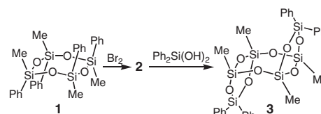
Scheme 6. Preparation of tricyclic laddersiloxane 3 .
