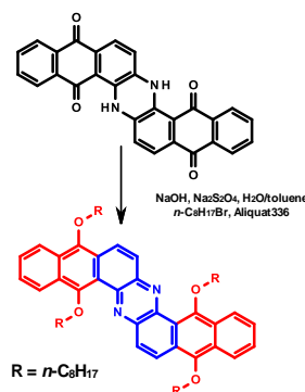
Scheme 1. Synthetic route to P-C8
