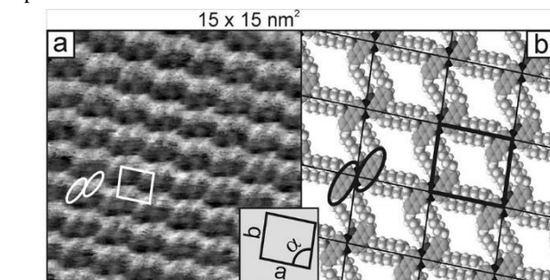
Figure 2. (a) STM image and (b) corresponding model of adsorption geometry of a monolayer of P-C8 deposited from hexane on HOPG graphite (15x15 nm 2 , I_t = 1 nA, V_{tip} = -1V ).
