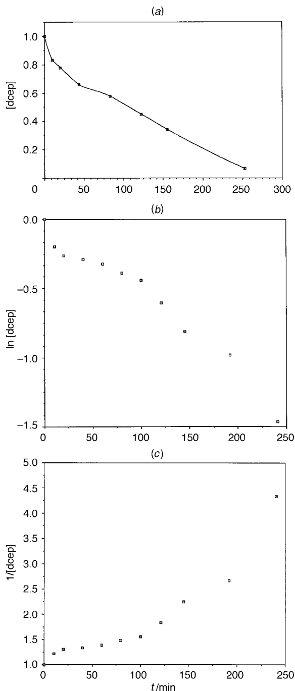
Fig. 2 (a) Plot of [dcep] [mole fraction of PH(CH 2 CH 2 CN) 2 ], determined from the integrals of spectra such as those in Fig. 1, against time, t . (b) A plot of ln[dcep] against time, t , illustrating that the kinetics are not first order and (c) a plot of 1/[dcep] against time, t , illustrating that the kinetics are not second order
