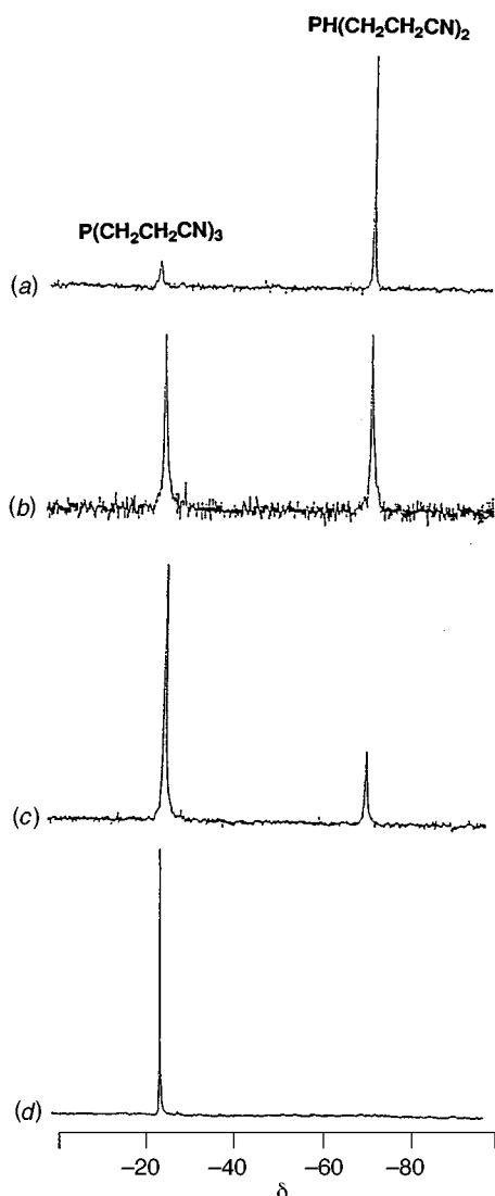
Fig. 1 Variation of ^{31}\text{P}\text{-}\{^1\text{H}\} NMR spectra with time upon addition of dcep to \text{CH}_2=\text{CHCN} in the presence of [\text{Pt}(\text{tcep})_3] under the standard conditions (see Experimental section) after (a) 10, (b) 120, (c) 240 and (d) 720 min
