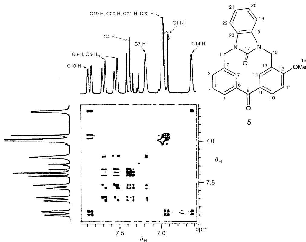
Fig. 8 ^1\text{H} - ^1\text{H} COSY spectrum of heterocalix[3]arene 5 .
