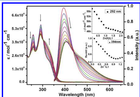
Figure 1. UV–vis and fluorescence titration spectra of ligand L1 with \text{Zn}(\text{ClO}_4)_2 in dichloromethane at 25 °C; the top inset shows the plot of molar extinction coefficient of 292 nm band as a function \text{Zn}(\text{II}) ion to L1 ratio; the bottom inset shows the plot of change in the fluorescence intensity at 394 nm, as a function of \text{Zn}(\text{II}) ion to L1 ratio. Arrows indicate the spectral changes with increasing amounts of \text{Zn}(\text{II}) ions.
