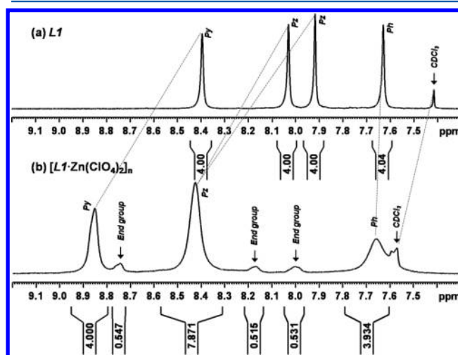
Figure 2. 1 H NMR (400 MHz, \text{CDCl}_3\text{-}d_1/\text{CD}_3\text{OD-}d_4 (3:2)) spectra 16 of (a) L1 and (b) polymer [\text{L1}\cdot\text{Zn}(\text{ClO}_4)_2]_n . TMS is used as a standard.
