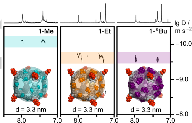
Figure 2. DOSY NMR spectra (600 MHz, C 2 D 2 Cl 4 or CDCl 3 , rt) for cages 1 (solvodynamic diameters are indicated as transparent spheres in the PM6-minimized [39] space-filling models, images have been prepared with PyMOL [40] ).
