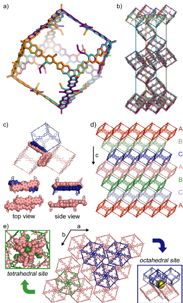
Figure 4. Overlay of a) monomers and b) unit cells for SC-XRD structures of cages 2-Me (turquoise), 2-Et (orange) and 2- n Bu (violet); fcc packing for 2-Me : c) two types of \pi - \pi -interactions between BDBA edges (rose/blue for interlayer and rose/rose for intralayer interactions), d) AB'CA'BC'-type layer stacking and e) top view for hexagonal layers (insets show the Me pockets at the tetrahedral sites (green box) and the extrinsic pore (yellow) at the octahedral sites (blue box), all images have been prepared with PyMOL [40] ).
