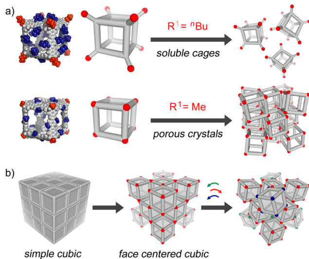
Figure 3. a) Control over solubility or crystallinity of cubic cages depending on substituents R 1 at the TBtQ vertices and b) schematic packing motifs for hollow cubic cages.
