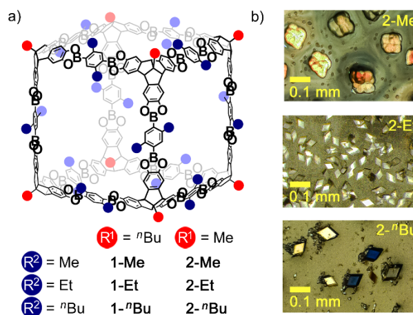
Figure 1. a) Chemical structure and substituents for cubic cages 1 and 2 and b) optical microscopy images of crystalline samples for cages 2.
