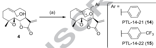
Scheme 3. Synthesis of C14-functionalized PTL analogs via O–H alkylation. (a) ArCH 2 Br, Ag 2 O, THF, room temperature, 24 hours.
