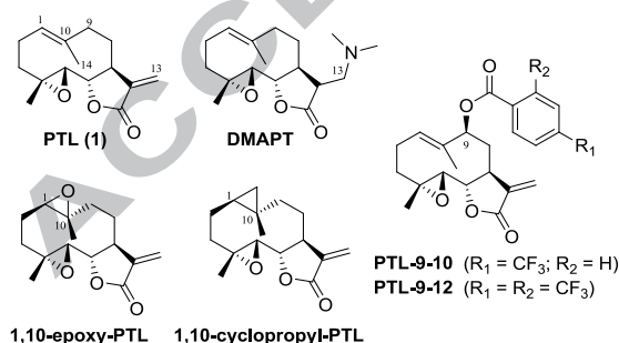
Figure 1. Chemical structure of parthenolide and previously reported parthenolide analogs.
