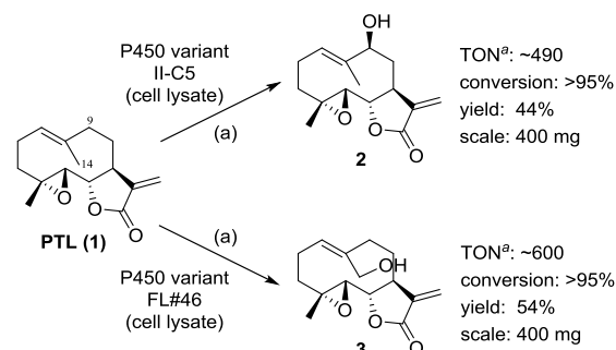
Scheme 1. Synthesis of 9( S )-hydroxy-parthenolide ( 2 ) and 14-hydroxy-parthenolide ( 3 ) via P450-catalyzed transformation of PTL. Reaction conditions: 1 mM PTL, ~ 0.1 mol% P450, 2 μM PTDH, 150 μM NADP + , 50 mM sodium phosphite in 50 mM potassium phosphate buffer (pH 8.0), room temperature, 14 hours. a The representative values of catalytic turnovers (TON) correspond to the formation of the indicated hydroxylation product only. In both reactions, 1,10-epoxy-parthenolide is also produced.
