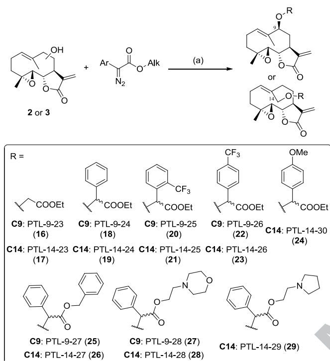
Scheme 4. Synthesis of C14-functionalized PTL analogs via O-H carbene insertion. (a) 5mol% Rh_2(OAc)_4 in dichloromethane, room temperature, 2 hours.
