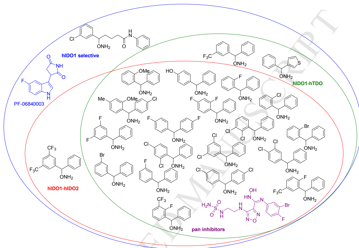
Figure 2. Venn diagram of selectivities seen with diaryl hydroxylamines in cell-based assay.
