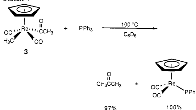
Scheme V
