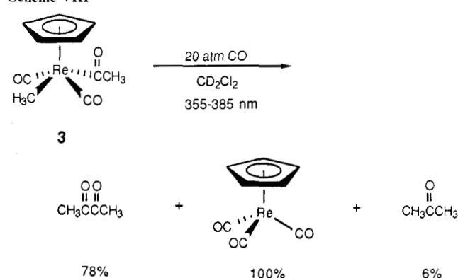
Scheme VIII
