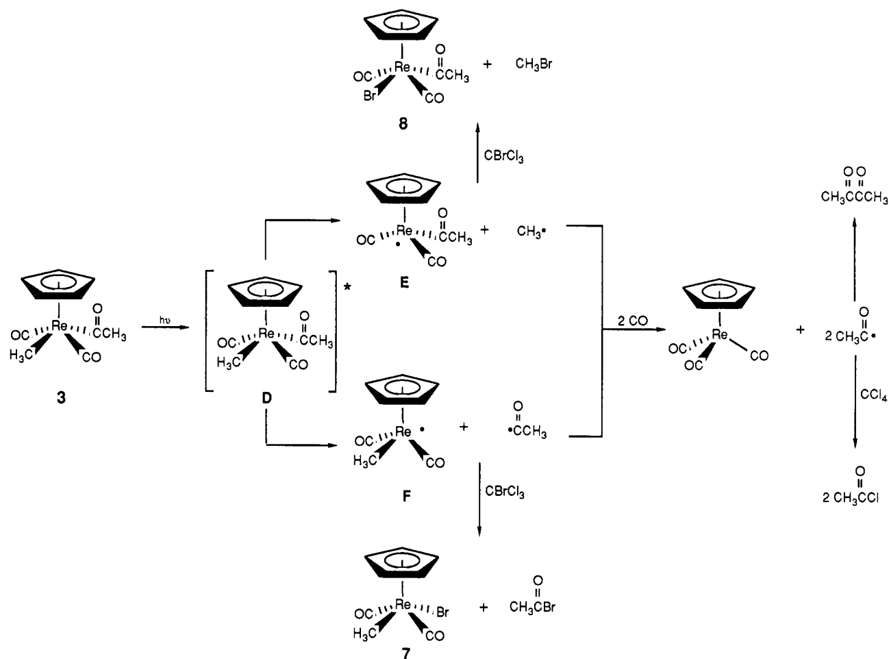
Scheme XVII
