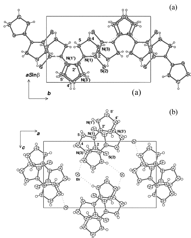
Fig. 3 Projections of the unit cell contents of 2 (a) and 2 ·HBr (b) down the c - (7.7913 Å) and b - (6.8957 Å) axes respectively.
