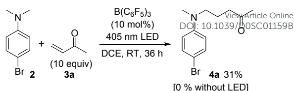
Scheme 2 Trapping experiment of \alpha -aminomethyl radical generated from 2 with 3a .
