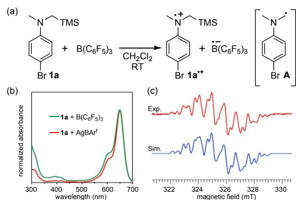
Fig. 1 (a) SET from 1a to B(C_6F_5)_3 . (b) UV-vis absorption spectra of the mixture of B(C_6F_5)_3 and 1a (green), and AgBAR^f and 1a (red). (c) Experimentally obtained ESR spectrum in CH_2Cl_2 (red) and a simulated spectrum of 1a •+ (blue).
