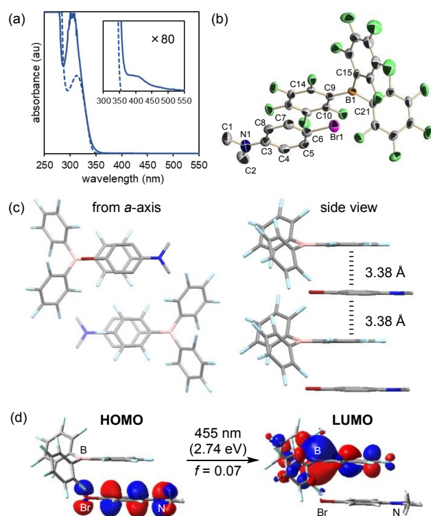
Fig. 3 (a) UV-vis spectra of a 1:1 mixture of B(C_6F_5)_3 and 2 (solid line) and 2 (hashed line) for 1.0 \cdot 10^{-3} M with magnified spectra (inner square). (b) X-ray structure of co-crystal of B(C_6F_5)_3 and 2 . (c) Packing structure of co-crystal of B(C_6F_5)_3 and 2 . (d) TD-DFT calculated minimum excitation of the single complex in crystal structure (CAM-B3LYP/6-311+G(d,p)).
