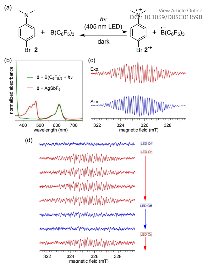
Fig. 2 (a) Photoinduced reversible SET between B(C_6F_5)_3 and 2 . (b) UV-vis spectra of a 1:1 mixture of B(C_6F_5)_3 and 2 after LED light irradiation and AgSbF_6 (red). (c) ESR spectrum after 1 h irradiation with a LED light (red) and a simulated spectrum (blue). (d) LED on/off ESR monitoring experiment of B(C_6F_5)_3 and 2 in CH_2Cl_2 . The interval of each measurement is 9 min.
