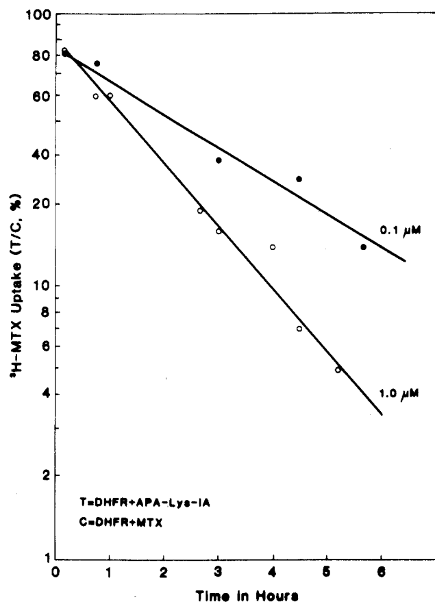
Figure 1. Decreased binding of [ ^3\text{H} ]MTX to L. casei DHFR following incubation with compound 1.
