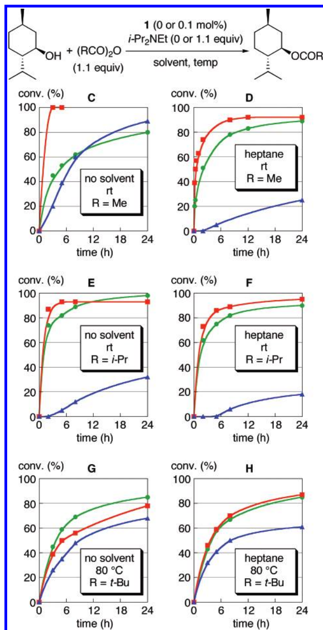
Figure 3. Effect of auxiliary base on the DMAP-catalyzed acetylation, isobutyrylation, and pivaloylation of l -menthol with acid anhydride. The reaction of l -menthol (5 mmol) was conducted with (\text{RCO})_2\text{O} (5.5 mmol) under solvent-free conditions or in heptane (5 mL); red squares, 1 (0.1 mol %) and i -Pr 2 NEt (1.1 equiv); green circles, 1 (0.1 mol %) without i -Pr 2 NEt; blue triangles, i -Pr 2 NEt (1.1 equiv) without 1 .
