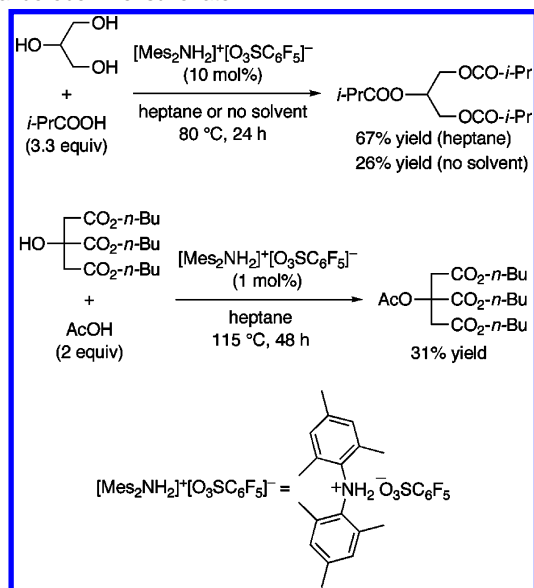
Scheme 1. Ester Condensation of Glycerol and Tributyl Citrate Catalyzed by N,N -Dimesitylammonium Pentafluorobenzensulfonate
