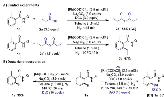
Scheme 4 Mechanistic studies.
