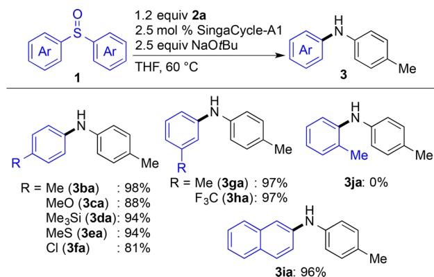
Scheme 2. Scope of Diaryl Sulfoxides
