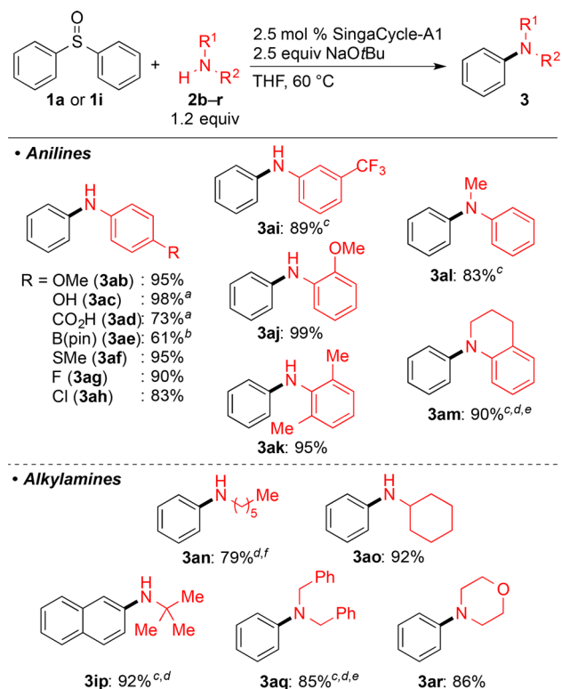
Scheme 1. Scope of Anilines and Alkylamines
