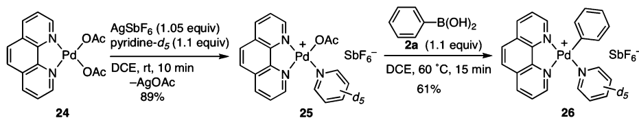
Scheme 6. Preparation of ( \sigma -Phenyl)palladium(II) Complex 26 and Its Stoichiometric Reaction with Allylic Acetate 1a
