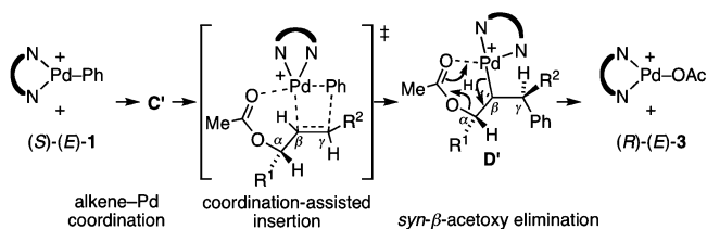
Scheme 9. Proposed Mechanism for the 1,3- syn Chirality Transfer for the Reaction between ( S )-( E )- 1 and 2a
