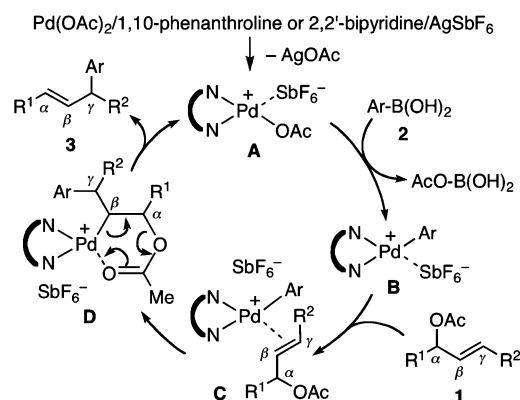
Scheme 8. Proposed Catalytic Cycle
