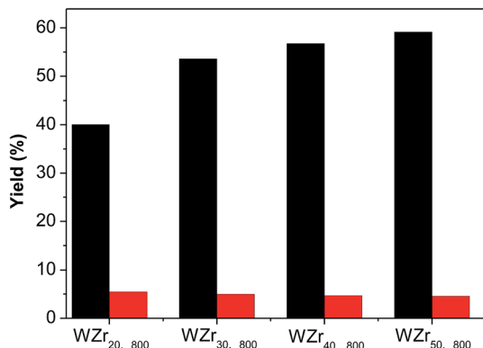
Fig. 9 The EG (black) and PG (red) yields obtained over the samples loading different amounts of \text{WO}_3 and being calcined at 800^\circ\text{C} (reaction conditions: 0.3 g cellulose, 0.01 g Ru/C, 0.08 g \text{WZr}_{x,800} , 40 mL \text{H}_2\text{O} , 215^\circ\text{C} , 5.2 MPa, 1000 rpm, 1.5 h).
