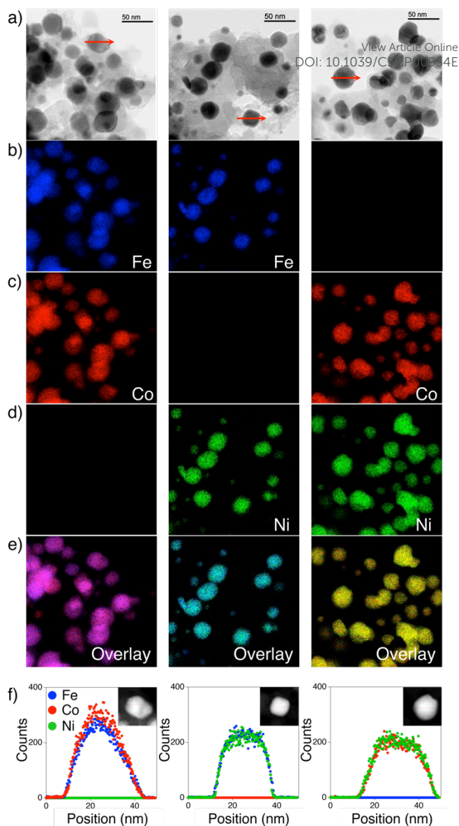
Fig. 1. (a) BF-STEM images and EDX composition maps of the (b) Fe-K \alpha (blue), (c) Co-K \alpha (red), (d) Ni-K \alpha (green) lines, (e) reconstructed overlay maps, and (f) EDX line-scan analysis results of (left) FeCo/C , (middle) FeNi/C , and (right) CoNi/C . Line scans were performed along the arrows marked in (a).
