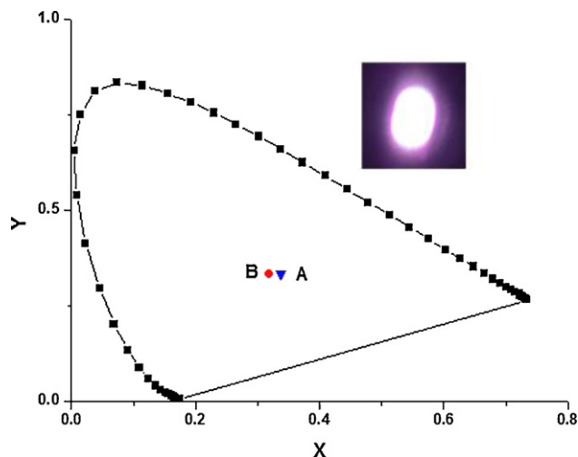
Fig. 8. CIE chromaticity diagrams of 1931 together with the calculated color coordinates for (A) \alpha\text{-TeO}_2\cdot\text{Tm}^{3+}/\text{Er}^{3+}/\text{Yb}^{3+} (0.5/0.25/10 mol%) nanoparticles and (B) \beta\text{-TeO}_2\cdot\text{Tm}^{3+}/\text{Er}^{3+}/\text{Yb}^{3+} (0.5/0.25/10 mol%) nanoparticles.
