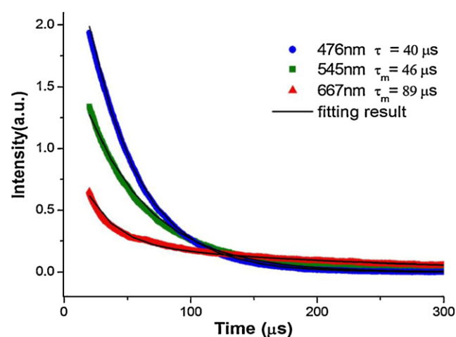
Fig. 6. Luminescence decay curves of blue (Tm 3+ : ^1G_4 \rightarrow ^3H_6 ), green (Er 3+ : ^4S_{3/2} \rightarrow ^4I_{15/2} ) and red (Er 3+ : ^4F_{9/2} \rightarrow ^4I_{15/2} ) emissions of \alpha -TeO 2 :Tm 3+ /Er 3+ /Yb 3+ (0.5/0.25/10 mol%) nanoparticles under 980 nm excitation.
