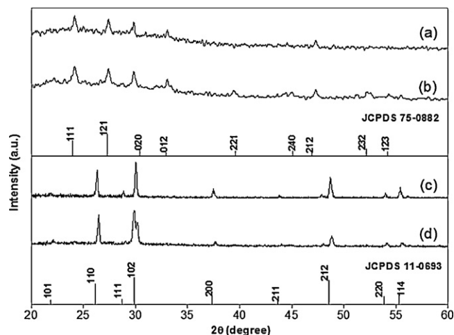
Fig. 1. XRD patterns of (a) \beta - \text{TeO}_2 : \text{Tm}^{3+}/\text{Er}^{3+}/\text{Yb}^{3+} (0.5/0.25/10 mol%) nanoparticles, (b) \beta - \text{TeO}_2 nanoparticles, (c) \alpha - \text{TeO}_2 : \text{Tm}^{3+}/\text{Er}^{3+}/\text{Yb}^{3+} (0.5/0.25/10 mol%) nanoparticles, and (d) \alpha - \text{TeO}_2 nanoparticles.
