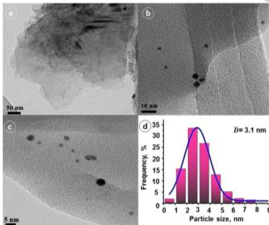
Figure 3. TEM images of bento-crt@Pd in different magnification (a-c). The solid curve is Gaussian fit to the data (d).
