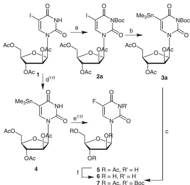
Scheme 1 Reagents and conditions: (a) (Boc) 2 O, DMAP, THF, 50%; (b) Sn 2 Me 6 , (PPh 3 ) 2 PdCl 2 , dioxane, 80 °C, 30%; (c) Selectfluor, MeCN, 50 °C, 50%; (d) 75%; (e) 30%; (f) NaOMe, MeOH, 95%.
