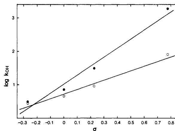
Figure 3. Plots of \log k_{\text{OH}} (M -1 s -1 ) vs \sigma , the Hammett substituent constant, for hydrolysis of substituted phenyl cinnamate esters (O) and plots of \log k_{\text{OH}} - 5 (M -1 s -1 ) vs \sigma for cyclization of the substituted phenyl esters of \alpha -acetamidocinnamic acid (III-VI) in 50% dioxane-H 2 O (v/v) at 50 °C and \mu = 0.1 M.
