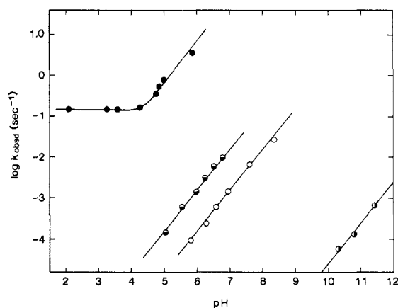
Figure 7. Plots of \log k_{\text{obsd}} vs pH for cyclization of 6-carboxy-2-pyridylmethyl \alpha -( N -acetyl-amino)cinnamate at 30^\circ\text{C} ( \mu = 0.1 \text{ M} ) in \text{H}_2\text{O} in the presence of saturating concentrations of \text{Cu}^{2+} ( 0.001 \text{ M} ) (●) and \text{Ni}^{2+} ( 0.004 \text{ M} ) (●) and in the absence of metal ion (○). Also shown is the plot of \log k_{\text{obsd}} vs pH for hydrolysis of 2-pyridylmethyl cinnamate (○). The ester concentration was 2 \times 10^{-5} \text{ M} .
