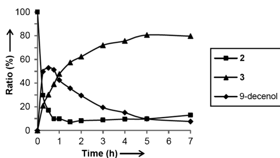
Figure 2. Time-course experiment monitoring relative amounts of 2 , 9-decenol, and the desired pheromone 3 .
