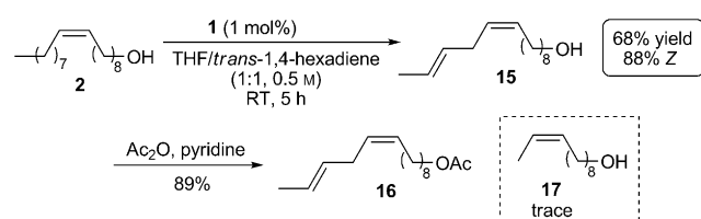
Scheme 4. Synthesis of pheromone 16 .
