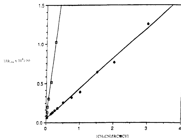
Figure 4. A plot of 1/(k_{\text{obs}} \times 10^4) versus [\text{MeCN}]/[\text{HC}\equiv\text{CR}] : (□) R = CO 2 Me, r^2 = 0.998 ; (◇) R = C(Me) 3 , r^2 = 0.993 .
