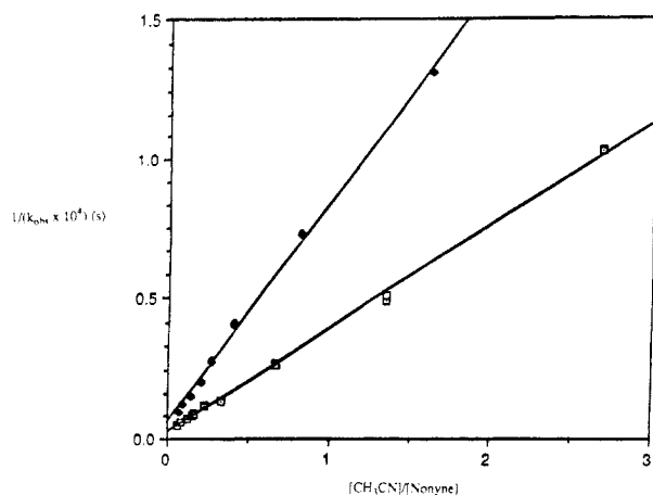
Figure 5. A plot of 1/(k_{\text{obs}} \times 10^4) versus [\text{MeCN}]/[\text{nonyne}] : ( \diamond ) 1-nonyne-1- d , r^2 = 0.998 ; ( \square ) 1-nonyne, r^2 = 0.998 .
