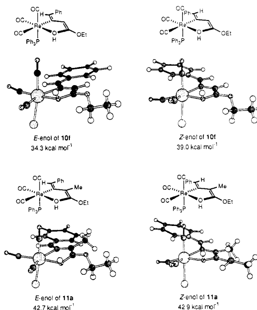
Figure 3. PCMODEL-generated minimum conformations and MMX energies for the enols of 10f and the E enol of 11a ; phenyl rings of the Ph 3 P ligands are omitted for clarity.
