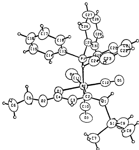
Figure 1. ORTEP diagram of alkyne addition product 10g with 50% probability thermal ellipsoids. The diagram shows the numbering scheme used in the tables.
