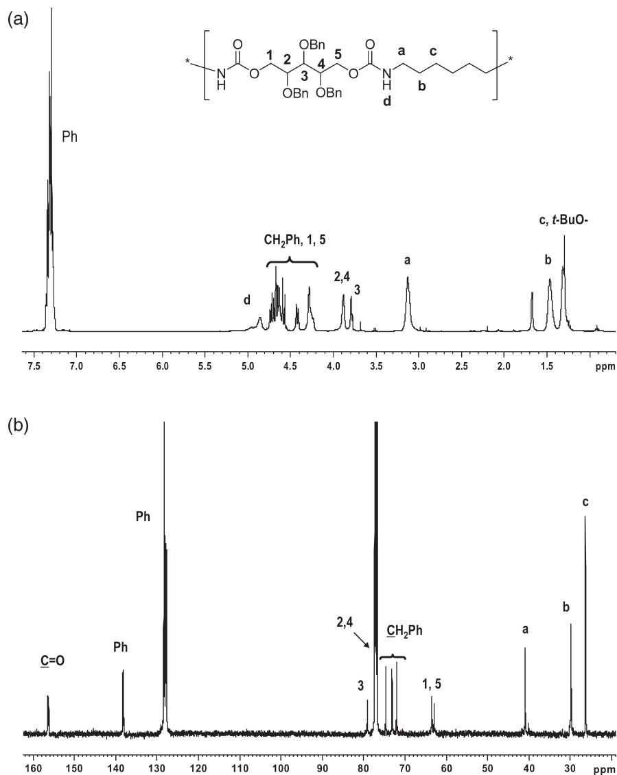
Figure 1: NMR spectra of polyurethane PU-ABnOH-HMDI in CDCl 3 . A: 1 H NMR spectrum; B: 13 C NMR spectrum.
