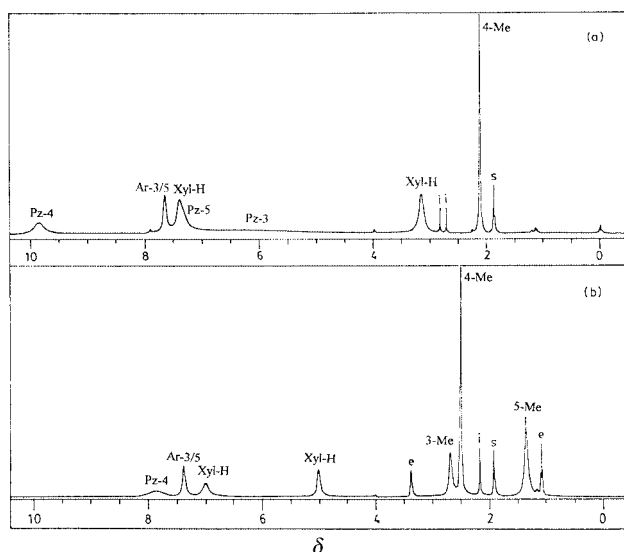
Fig. 3 400 MHz ^1\text{H} NMR spectra of (a) [\text{Cu}_2(\text{L})_2(\text{OCIO}_3)_2] 1 and (b) [\text{Cu}_2(\text{L}')_2(\text{OCIO}_3)_2] 2 at room temperature in \text{CD}_3\text{CN} solution. The peaks marked e, i and s are due to diethyl ether, impurity and solvent, respectively. The abbreviations (Ar, Pz and Xyl) used in the assignments denote aromatic ring, pyrazole ring and xylyl protons respectively.
