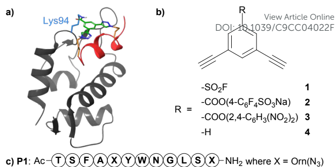
Fig. 1 a) Molecular dynamics simulation of PMI-derived stapled peptide (red) covalently linked with MDM2 (grey) through amide bond with Lys94 close to the binding site. b) The structures of the proposed staples: aryl sulfonyl fluoride 1 , sulfotetrafluorophenyl (STP) ester 2 , and dinitrophenyl ester 3 . The non-electrophilic staple 4 was used as a control. c) The optimal linear diazidopeptide P1 .
