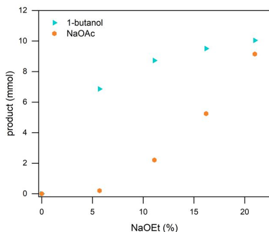
Figure 2. The formation of undesirable NaOAc can be virtually eliminated by decreasing the NaOEt content. Results are shown for reactions with 2 after 14.5 h at 170 °C.
