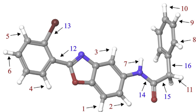
Fig. 9. BDEs of all single acyclic bonds of N -[2-(2-bromophenyl)-1,3-benzoxazol-5-yl]-2-phenyl acetamidemolecule
