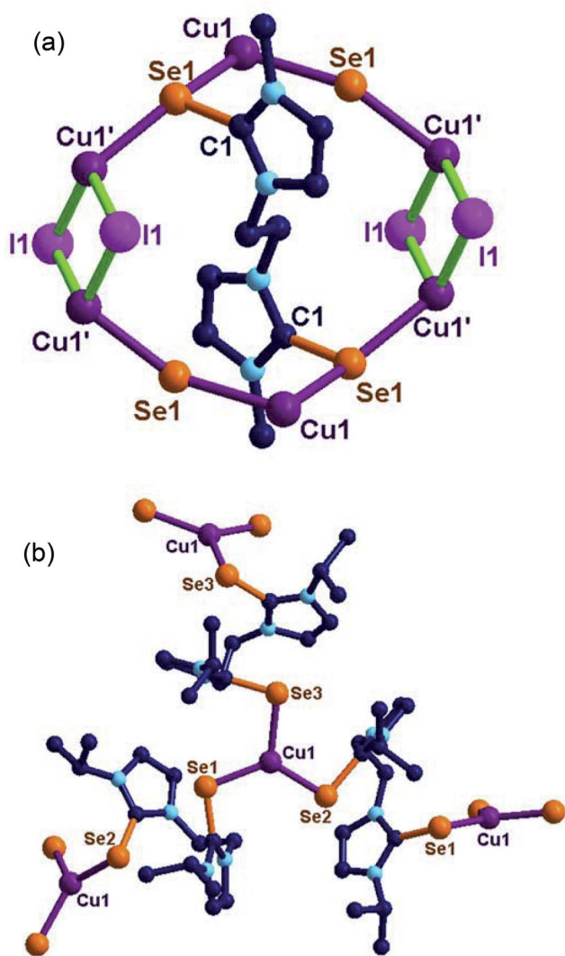
Fig. 4 (a) Solid-state structure of 13 . Selected bond lengths (Å) and angles (°): C(1)–Se(1), 1.867(7), Se(1)–Cu(1), 2.553(14), Cu(1)–I, 2.650(12), Cu(1')–I, 2.660(13), C(1)–Se(1)–Cu(1), 95.3(2), C(1)–Se(1)–Cu(1'), 103.4(2), N(1)–C(1)–N(2), 106.8(6), N(1)–C(1)–Se(1), 127.3(5), N(2)–C(1)–Se(1), 125.9(5), Cu(1)–Se(1)–Cu(1'), 160.72(10). (b) Solid state structure of 14 . Selected bond lengths (Å) and angles (°): C(1)–Se(1), 1.859(5), Se(1)–Cu(1), 2.336(9), C(8)–Se(2), 1.874(5), Se(2)–Cu(1), 2.323(10), C(15)–Se(3), 1.842(10), Se(3)–Cu(1), 2.352(10), C(1)–Se(1)–Cu(1), 102.35(15), C(8)–Se(2)–Cu(1), 99.85(16), C(15)–Se(3)–Cu(1), 98.6(3), Se(1)–Cu(1)–Se(2), 126.86(4), Se(1)–Cu(1)–Se(3), 114.60(4), Se(2)–Cu(1)–Se(3), 118.49(4), N(1)–C(1)–N(2), 106.0(5), N(1)–C(1)–Se(1), 125.6(4), N(2)–C(1)–Se(1), 128.3(4), N(3)–C(8)–N(4), 106.0(5), N(3)–C(8)–Se(2), 127.1(4), N(4)–C(8)–Se(2), 126.9(4), N(5)–C(15)–N(6), 108.7(12), N(5)–C(15)–Se(3), 125.1(10), N(6)–C(15)–Se(3), 126.2(11).
