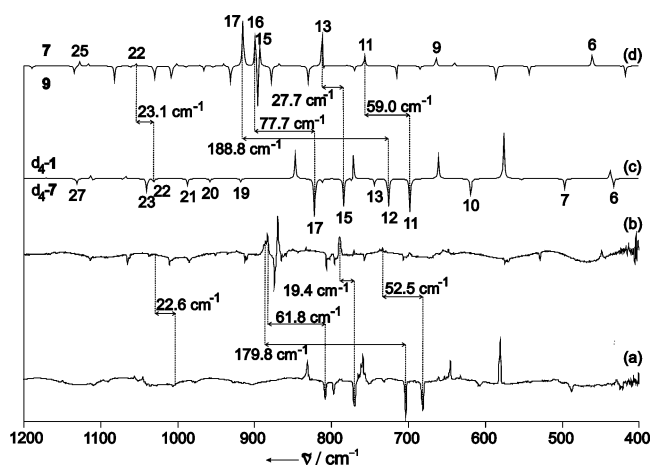
Figure 6. Difference IR spectra showing the photochemical interconversion of 1, 7, and 9 in argon at 10 K. The experimental difference spectra are compared to simulated difference spectra based on calculations at the B3LYP/6-311G(d,p) level of theory. (a) \lambda = 254\text{ nm} irradiation converts d_4 -1 (disappearing, peaks pointing downward) into d_4 -7 (appearing, peaks pointing upward). (b) \lambda > 350\text{ nm} irradiation converts 9 (disappearing, peaks pointing downward) into 7 (appearing, peaks pointing upward). (c) Simulated difference spectrum d_4 -1– d_4 -7 corresponding to (a). (d) Simulated difference spectrum 7–9 corresponding to (b). The isotopic shifts of the exo -methylene groups of 7 are shown in the spectra.
