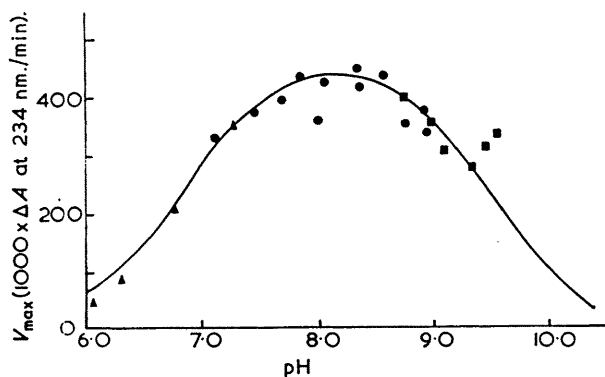
FIGURE 1. pH-Activity profile of lipoxygenase, using linoleyl sulphate as substrate. Comparison of experimental data with computed curve. Buffers used were, 0.1M-2-(N-morpholino)ethanesulphonic acid (triangles), 0.1M-Tris (circles), and 0.1M-glycine (squares). V_{\max} , the maximum activity, is expressed as 1000 \times absorbance change at 234 nm. in standard assay. See ref. 4 for details.
