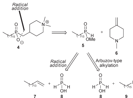
Scheme 1 Retrosynthetic analyses of 4.
