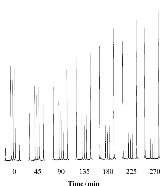
Fig. 4 Variation of the ^{31}\text{P} NMR spectrum with time for \text{D}_3\text{PO}_3 ( 0.10 \text{ mol dm}^{-3} ) in 0.75 \text{ mol dm}^{-3} \text{HClO}_4 , 55^\circ\text{C} , I = 1.0 \text{ mol dm}^{-3} ( \text{NaClO}_4 ). Every third spectrum shown.
