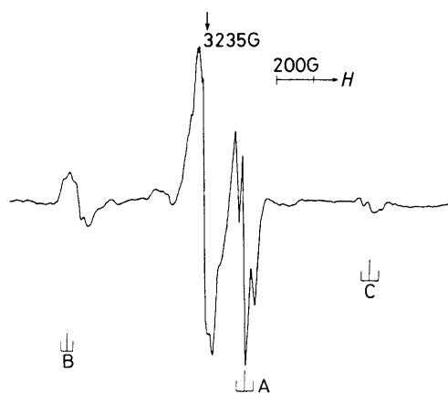
Figure 4. First-derivative X-band e.s.r. spectrum for a dilute solution of \text{Hg}(\text{C}_2\text{H}_5)_2 in \text{CFCl}_3 , showing the perpendicular feature assigned to \text{Hg}(\text{C}_2\text{H}_5)_2^{*+} cations, with a triplet splitting of 42 G assigned to hyperfine coupling to two equivalent protons. The extra central line is due to organic radicals
