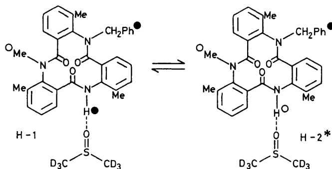
FIGURE 7 The H-1 \rightleftharpoons H-2* conformational equilibrium for compound (16) in hexadeuteriodimethyl sulphoxide
