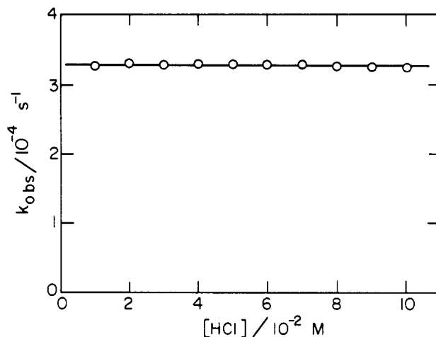
Figure 2. Relationship between acid concentration and specific rate of detritiation of tert -butylmalononitrile in aqueous HCl solutions at 25 °C.
