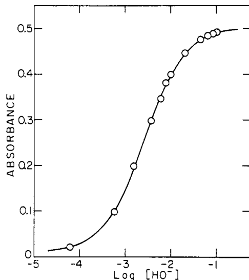
Figure 1. Spectrophotometric titration curve for the acid ionization of malononitrile in aqueous solution at 25 °C and ionic strength 0.10 M; the line shown was drawn with parameters obtained by least-squares fit to eq 3.
