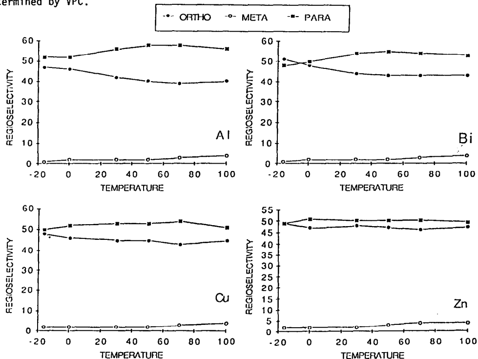
Fig. 1-4- Regioselectivities of ring nitration of toluene as a function of temperature (°C), using nitrates of Aluminum, Bismuth, Copper and Zinc respectively (other conditions as in Table 1). The expectation, based on earlier work on the nitration of halobenzenes 6 , was of a considerable dependence of the product distribution on temperature.
