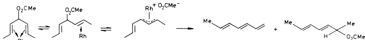
Scheme 2. Mechanism for the Rh I -catalysed conversion of ( E,E )-4-acetoxyhepta-2,5-diene into ( E,E )-hepta-1,3,5-triene and ( E,E )-2-acetoxyhepta-3,5-diene
