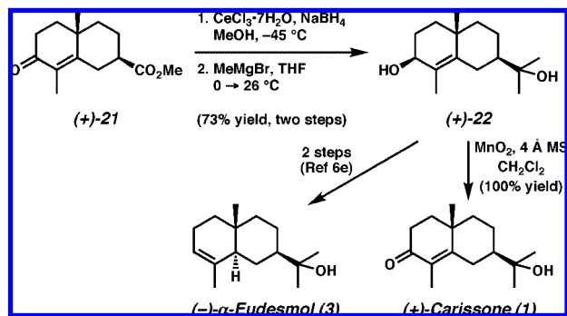
Scheme 3. End Game for (+)-Carissone ( 1 )
