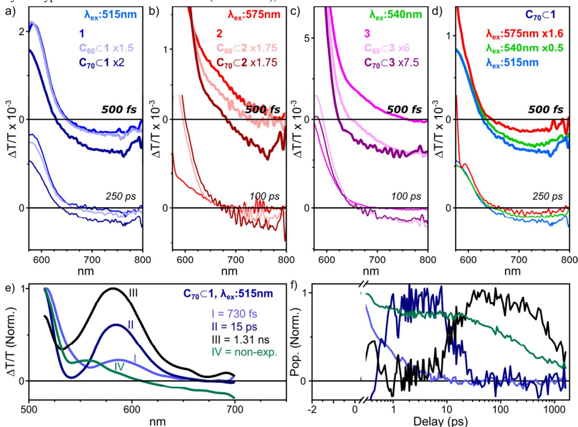
Figure 6. Spectroscopic signatures of host-guest interactions in fullerene-loaded BODIPY cages. TA spectra of (a) 1 , \text{C}_{60}<1 and \text{C}_{70}<1 following excitation at 515 nm; (b) 2 , \text{C}_{60}<2 and \text{C}_{70}<2 following excitation at 575 nm; and (c) 3 , \text{C}_{60}<3 and \text{C}_{70}<3 following excitation at 540 nm, revealing additional PIA ( \Delta T/T < 0 ) from charge-separated states which persist for hundreds of ps. (d) Pump-wavelength dependence of the fullerene charge-transfer signal for \text{C}_{70}<1 . A similar dependence was observed for \text{C}_{60}<1 , as well as for fullerene-loaded 2 and 3 (see Figures S26-S28). All data sets were scaled as indicated to account for excitation density. Full spectra are provided in the Supporting Information. (e) Spectral decomposition of TA data for \text{C}_{70}<1 , and (f) corresponding population kinetics. Species I-III display similar decay kinetics to those observed in the decomposition of empty 1 , with no direct relationship to charge-transfer species IV.
