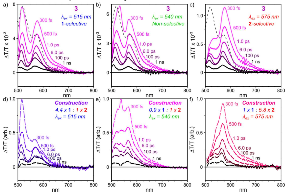
Figure 4. Strong coupling in heteroleptic cages. TA spectra of 3 at selected pump-probe delays, following excitation at (a) 515 nm, (b) 540 nm and (c) 575 nm. Dashed spectrum corresponds to UV-Vis absorption. (d-f) Synthetic TA spectra constructed from homoleptic cage data, based on differing relative contributions to overall UV-Vis absorption (ratio indicated). These constructed spectra fail to reproduce peak positions or relative intensities.
