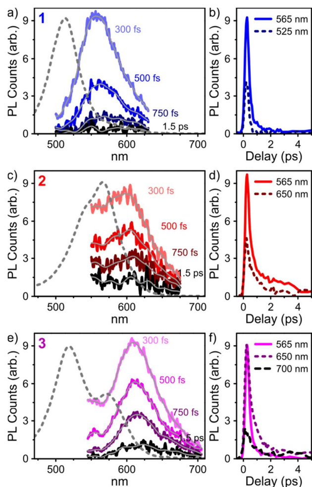
Figure 2. Ultrafast photoluminescence spectra and corresponding kinetics for films of (a, b) 1 , (c, d) 2 , and (e, f) 3 with <200-fs temporal resolution, at the delay times indicated in panels. Gray lines are smoothed as a guide to the eye. Dashed lines are UV-Vis absorption spectra from Figure 1. Excitation was carried out at 400 nm.
