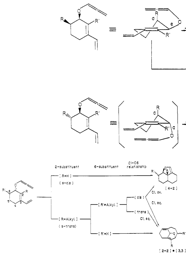
Figure 2. The structure-reactivity relationship in the intramolecular cycloaddition of allenyl ethers.
