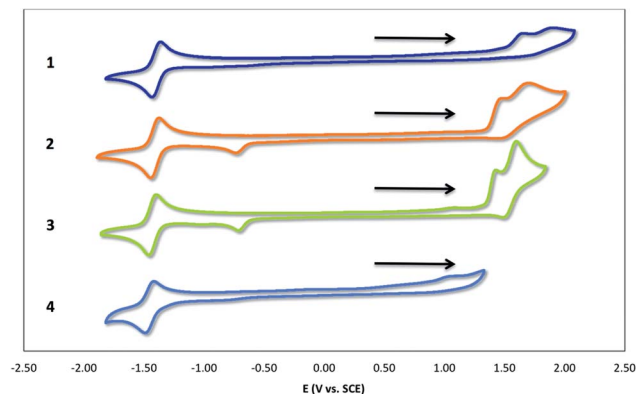
Fig. 1 Cyclic voltammetry for 1–4, recorded in deaerated acetonitrile; supporting electrolyte TBAPF 6 0.1 M. Working electrode: glassy carbon; counter electrode: Pt wire; reference electrode: Ag wire pseudo-reference. The Fc + /Fc couple was used as an internal standard and the potential was then referred to SCE ( E_{\text{SCE}} = E_{\text{Fc}^+/\text{Fc}} + 0.38 \text{ V} ). 16 — 1; — 2; — 3; — 4.
