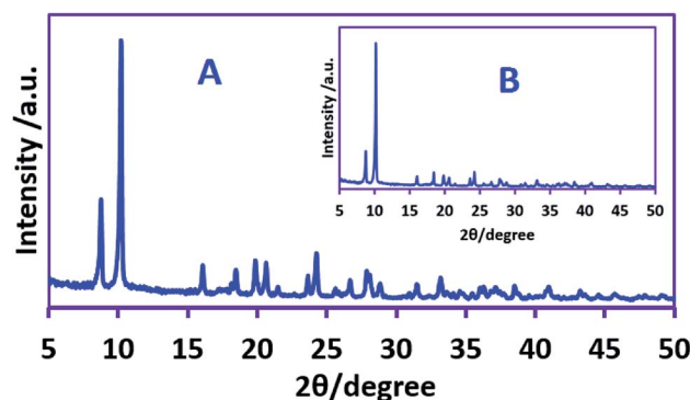
Fig. 3 XRD patterns of the AgSD synthesized at applied current density of: (A) 62.5 mA \text{cm}^{-2} and (B) 12.5 mA \text{cm}^{-2} .
