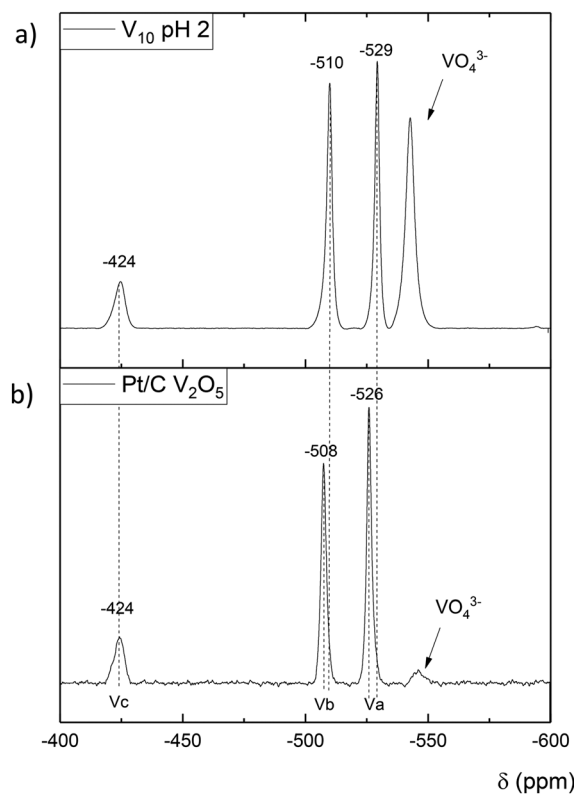
Fig. 5 ^{51}V NMR of a) vanadium decavanadate which is present at low pH with presence of monovanadate also b) reaction sample of Pt/C and V_2O_5 with 4000 ppm 2-HCO solution c) V_{10} compound with labelled vanadium sites corresponding to the shifts shown in the NMR spectra.
