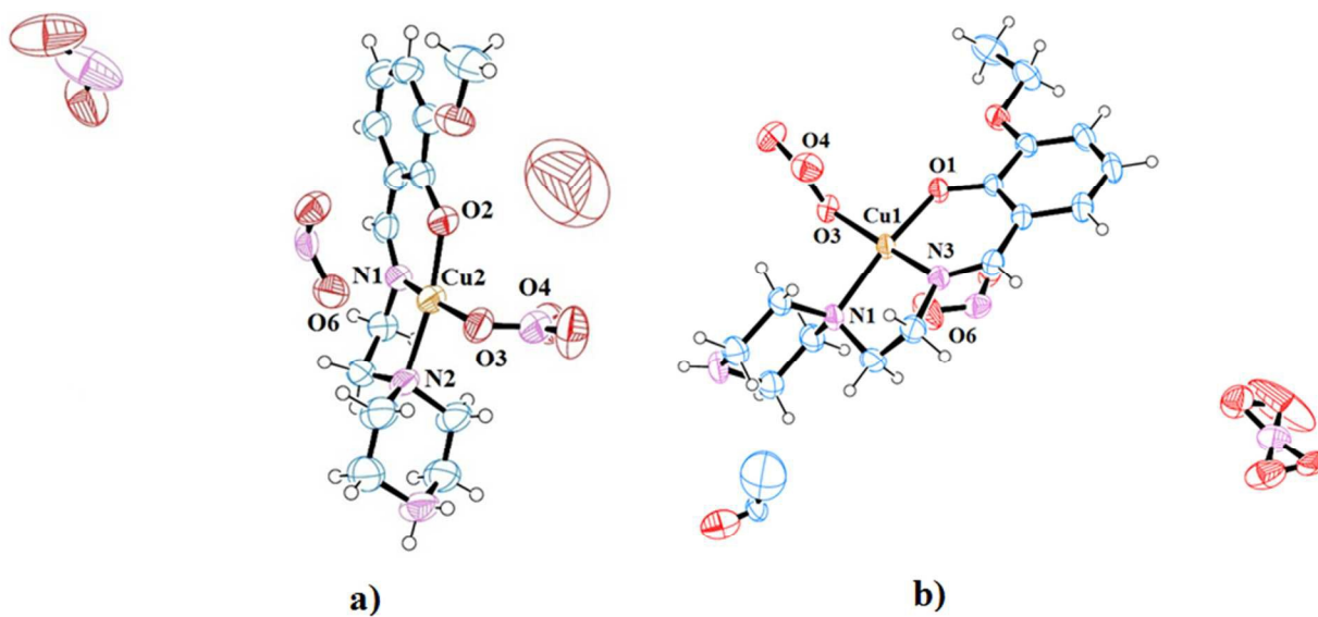
Fig. 1 ORTEP diagram of complexes 1 a) and 2 b)
